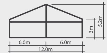
Type: 12m Span
