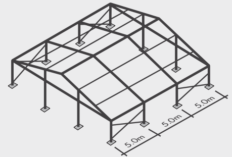
Type: 10m Span
