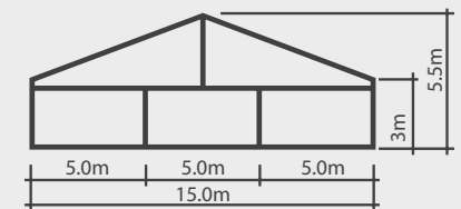
Type: 15m Span
