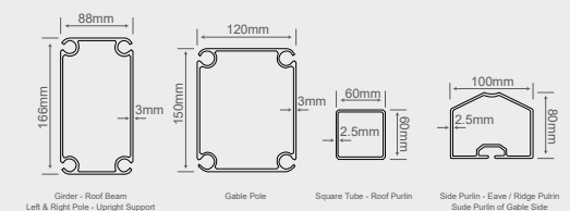
166 x 88 x 3mm Profile
