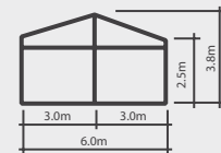
Type: Span 6m
