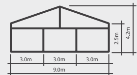
Type: Span 9m
