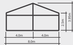
Type: Span 8m
