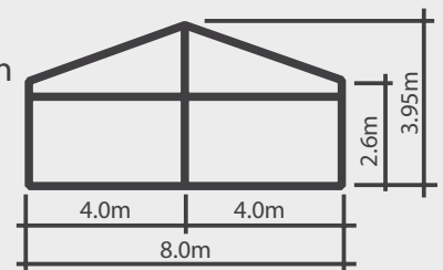
Type: 8m Span
