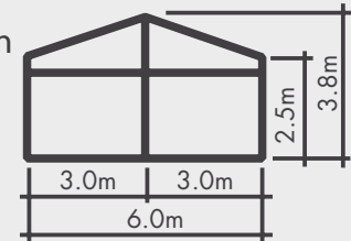
Type: 6m Span
